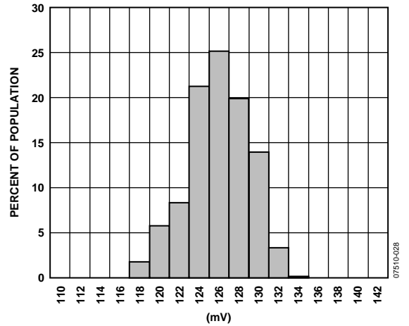
Figure 14. ADXL001-250, Self-Test Delta
