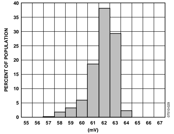
Figure 15. ADXL001-500, Self-Test Delta
