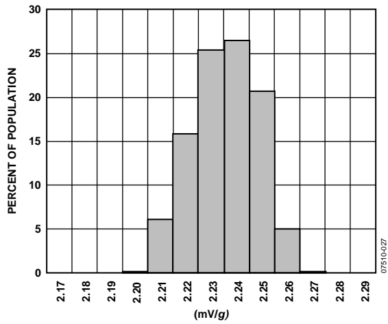
Figure 12. ADXL001-500, Sensitivity Distribution (TA = 125°C)
