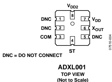
Figure 4. Pin Configuration
