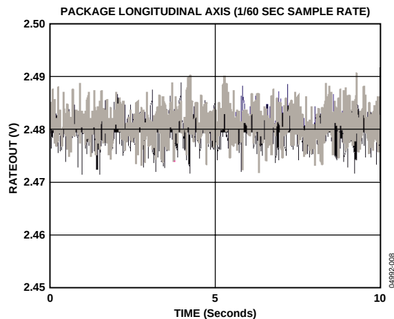
Figure 9. 10 g Random Vibration in Package-Longitudinal Axis Orientation
