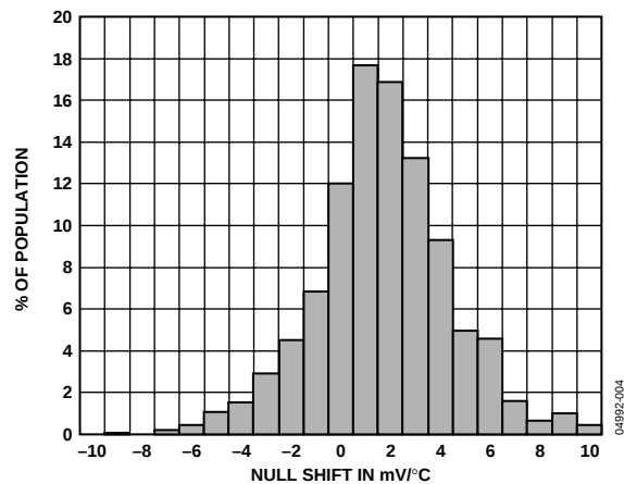
Figure 5. Null Tempco
