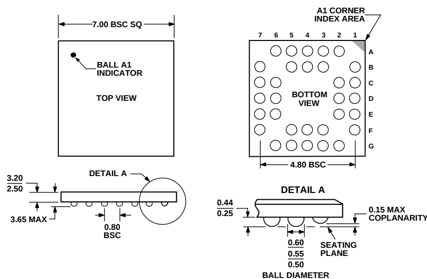
Figure 21. 32-Lead Chip Scale Ball Grid Array [CSPBGA] (BC-32) Dimensions shown in millimeters
