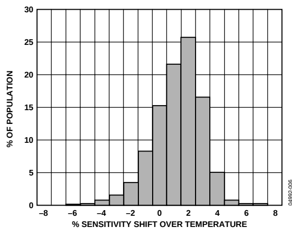
Figure 7. Sensitivity Change Over Temperature
