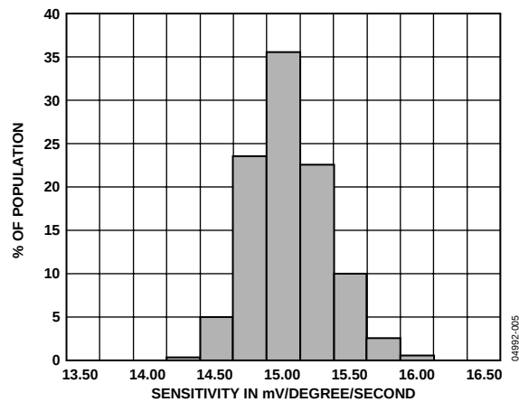
Figure 6. Initial Sensitivity
