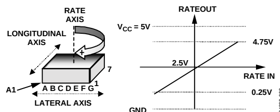
Figure 2. RATEOUT Signal Increases with Clockwise Rotation
