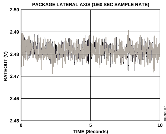
Figure 8. 10 g Random Vibration in Package-Lateral Axis Orientation
