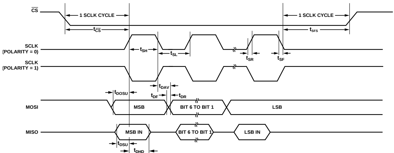
Figure 5. SPI Master Mode Timing (Phase Mode = 0)
