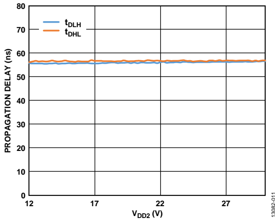
Figure 11. Typical Propagation Delay vs. Output Supply Voltage ( V_{DD2} ) for V_{DD2} = 15\text{ V} and V_{DD1} = 5\text{ V}
