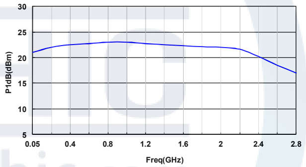
Frequency vs. P1dB
