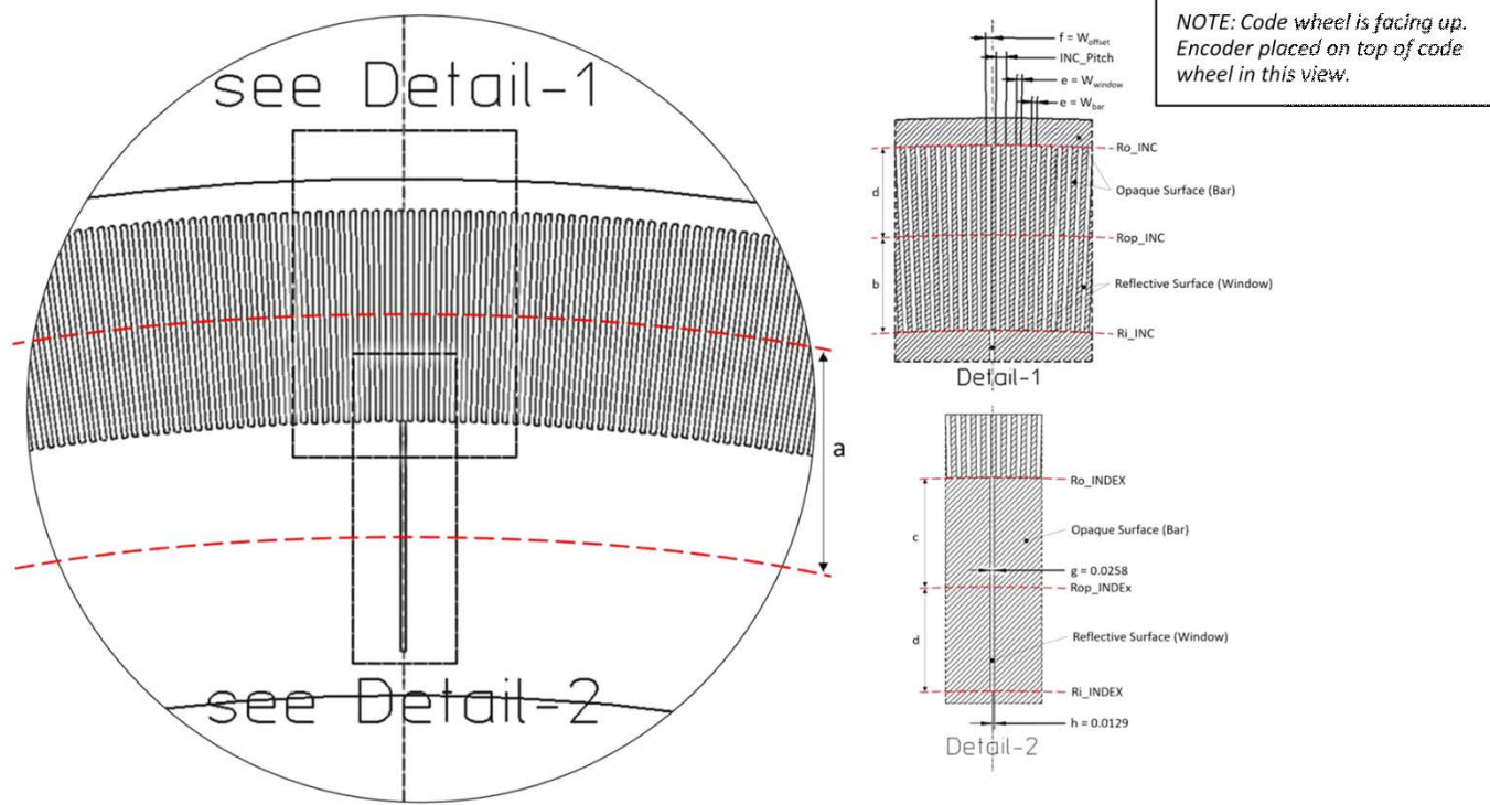
Figure 9: Code Wheel Design
