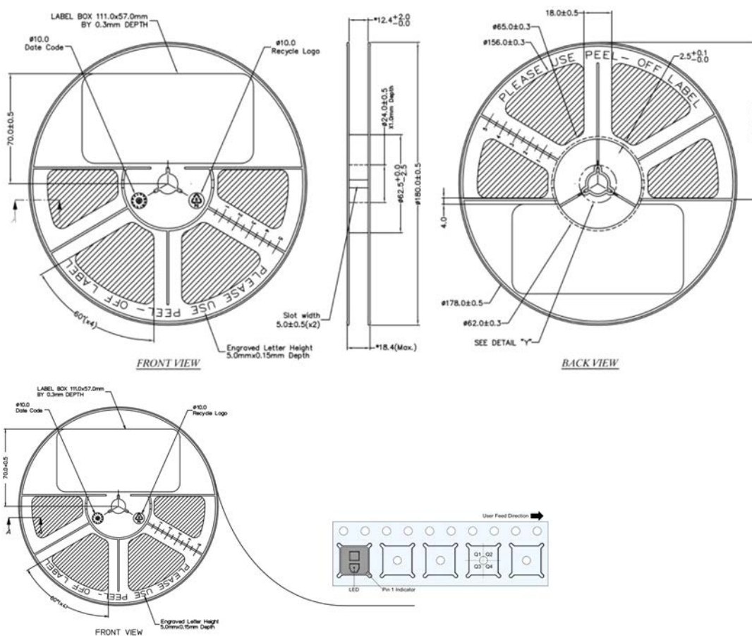
Figure 14: AEDR-9930E2 Reel Dimensions and Orientation
