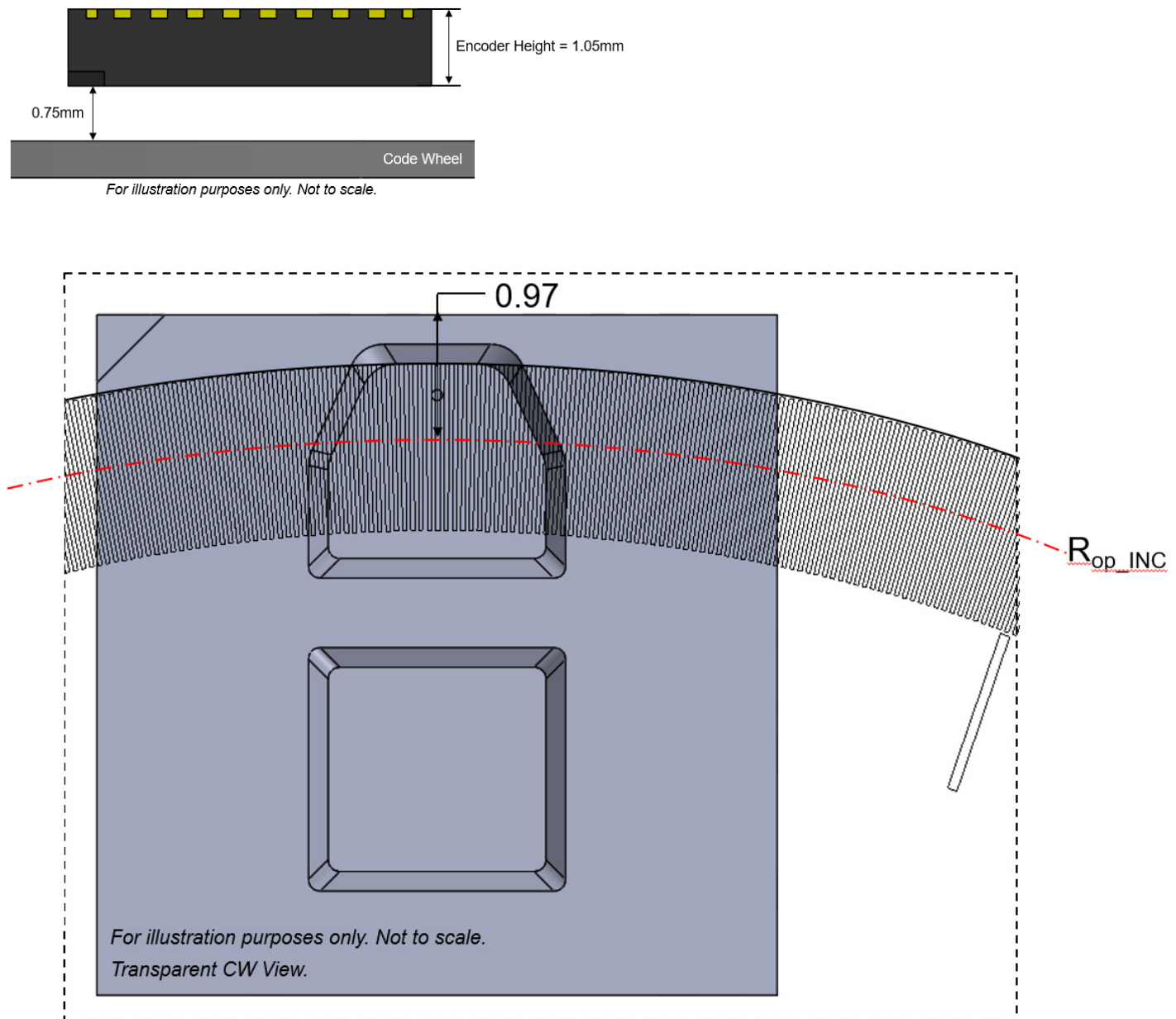
Figure 10: Top-Down View of the AEDR-9930E2 with Respect to Code Wheel Positioning
