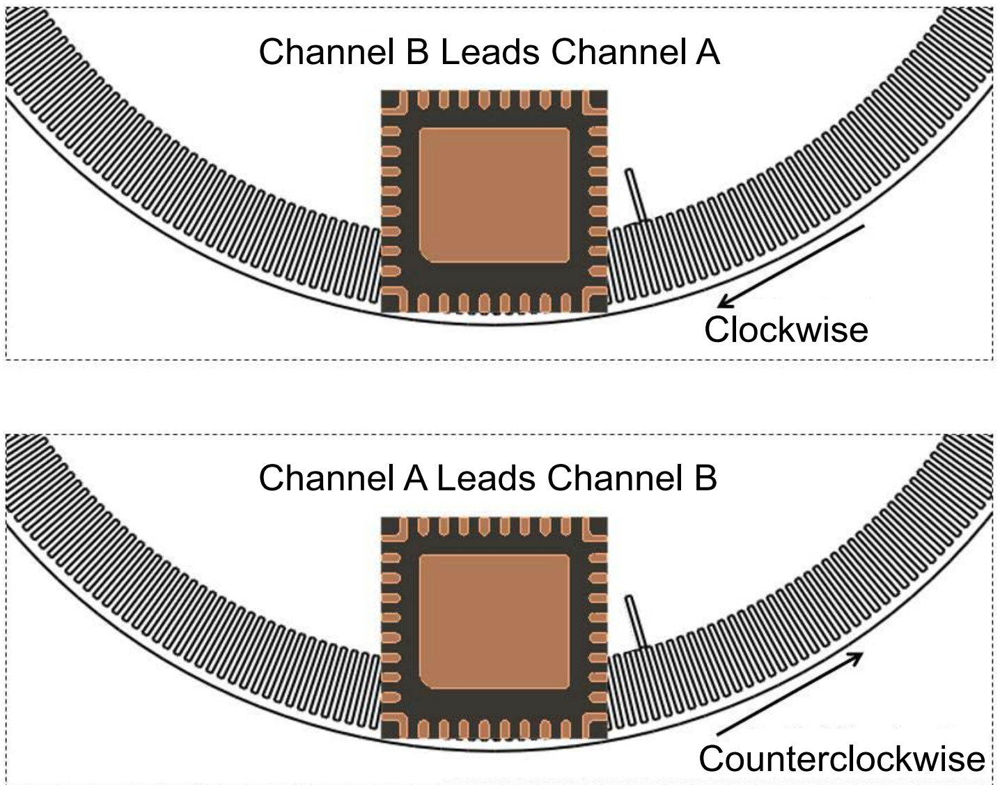
Figure 11: Channel A and Channel B Signal Output Sequence with Respect to Code Wheel Rotational Direction
