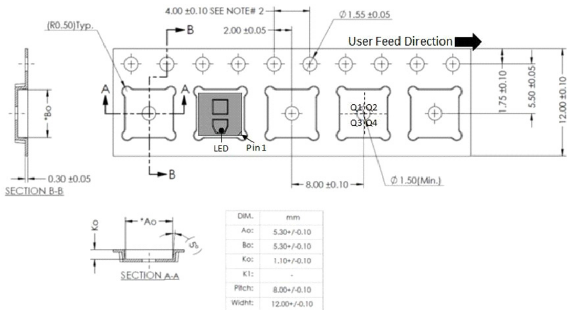
Figure 13: AEDR-9930E2 Carrier Tape Dimensions
