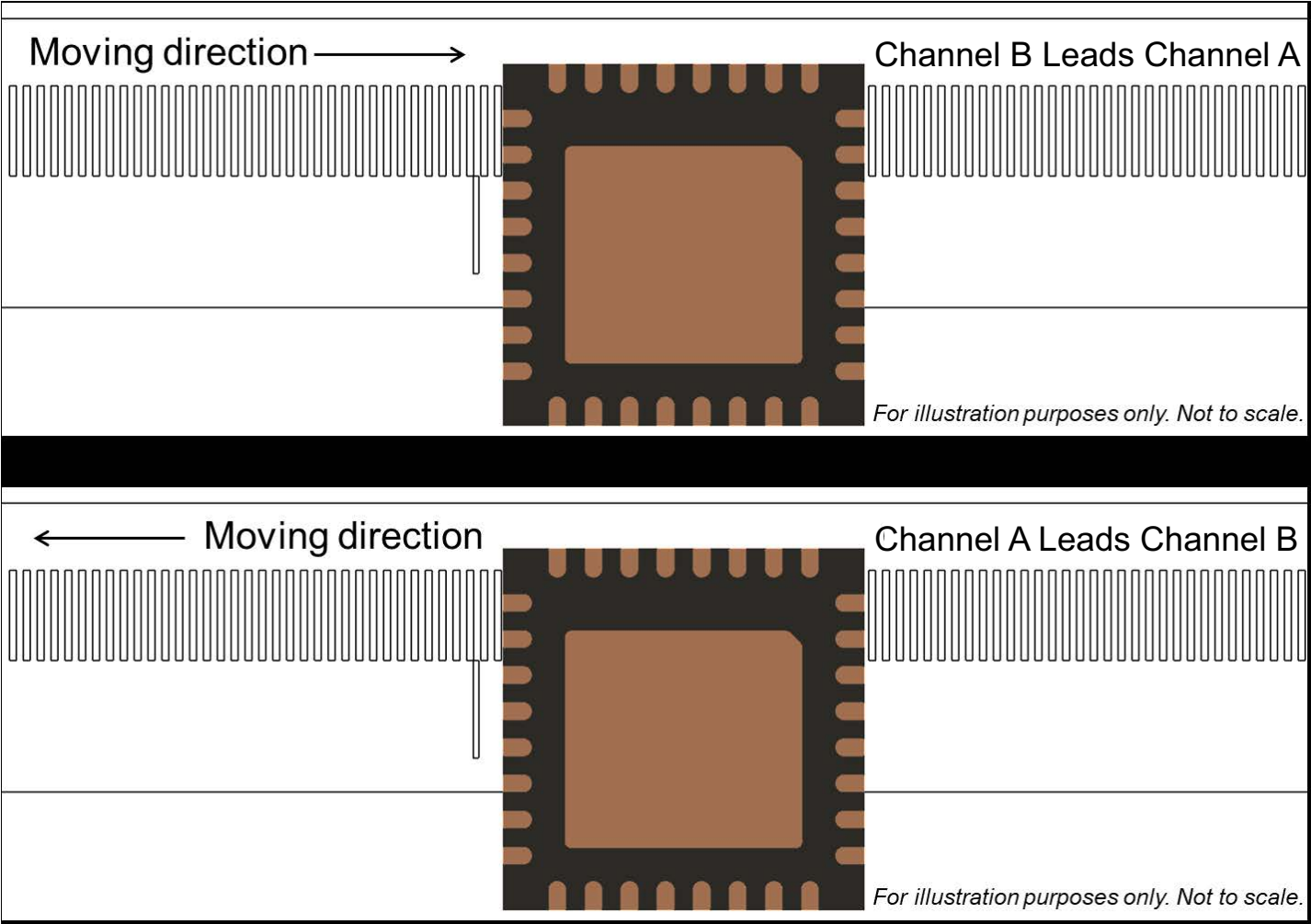
Figure 11: Channel A and Channel B Signal Output Sequence with Respect to Code Wheel Rotational Direction
