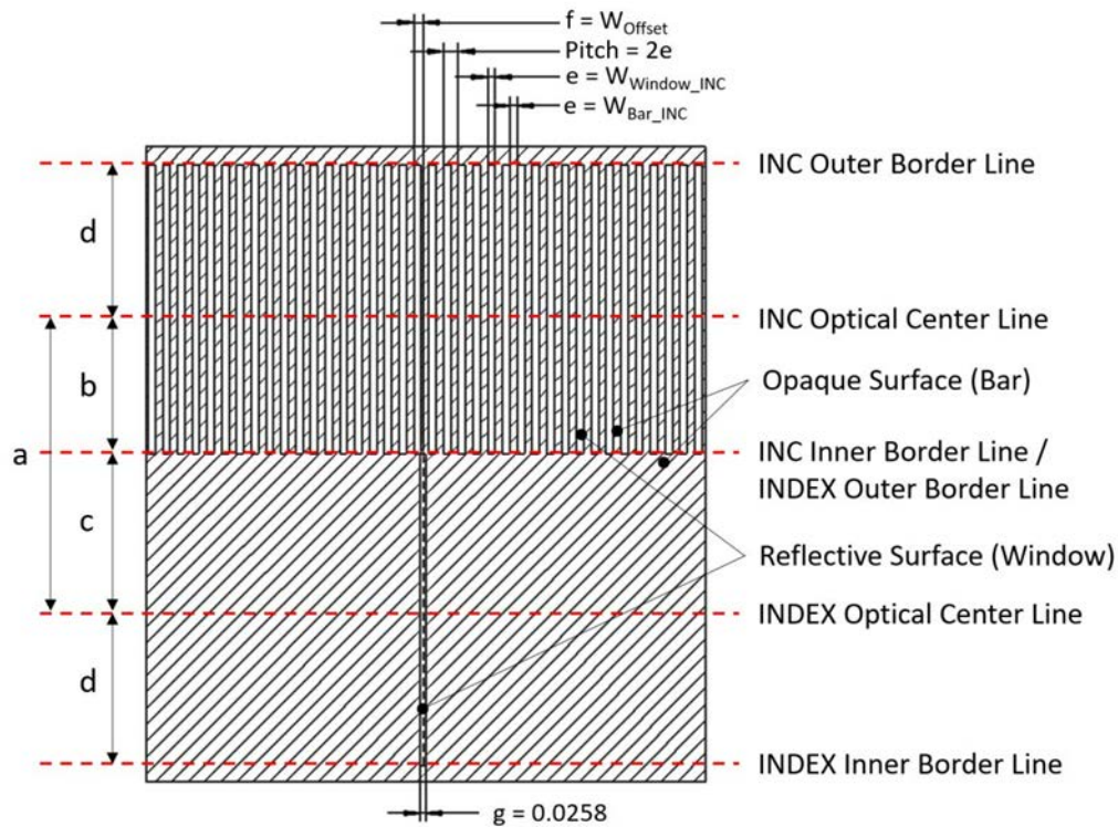
Figure 9: Code Strip Design
