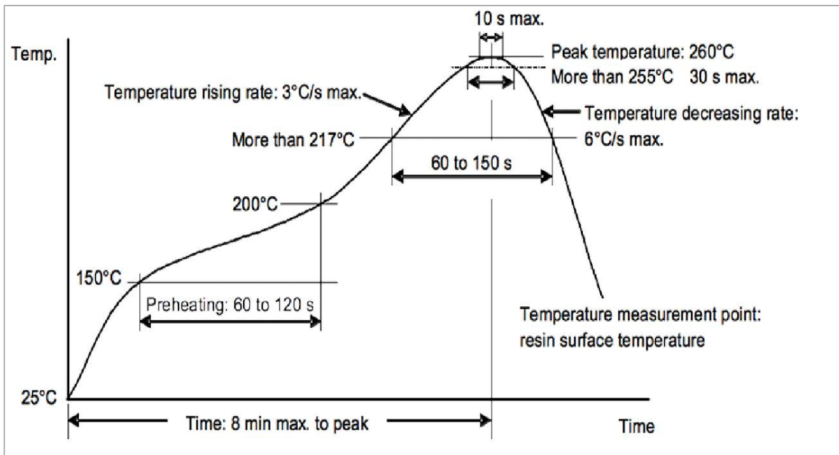
Figure 12: Typical Lead-Free Solder Reflow Profile
