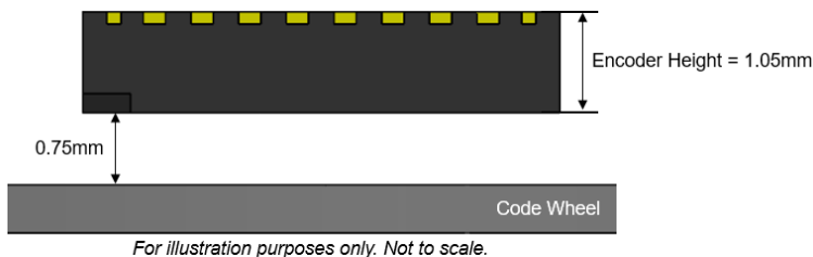
Figure 10: Top-Down View of the AEDR-9930E2L with Respect to Code Wheel Positioning
