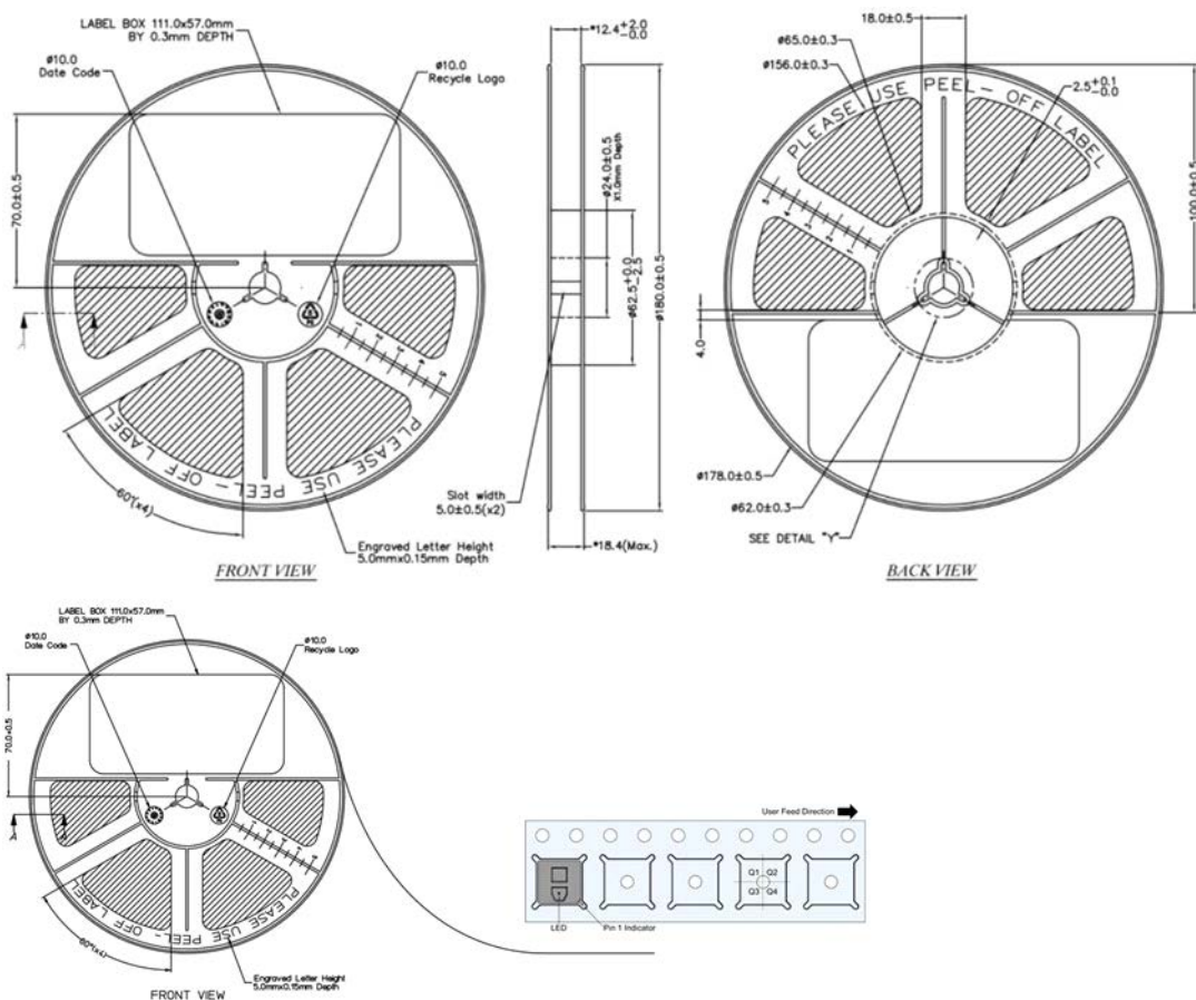
Figure 14: AEDR-9930E2L Reel Dimensions and Orientation
