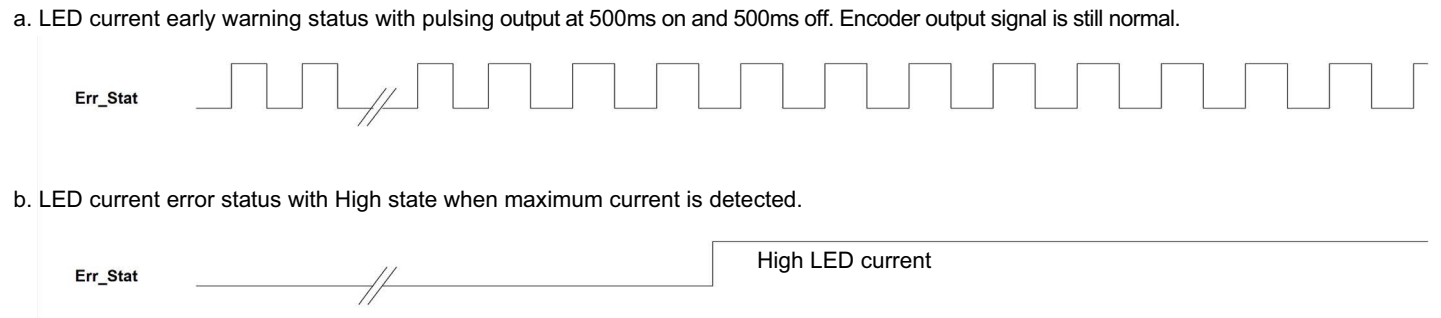
Figure 7: LED Error Status Pin
