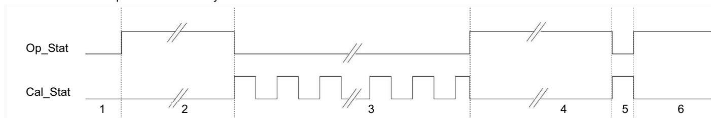
Figure 6: LED Status Pins Signals with Multiple Index Checks Enabled
