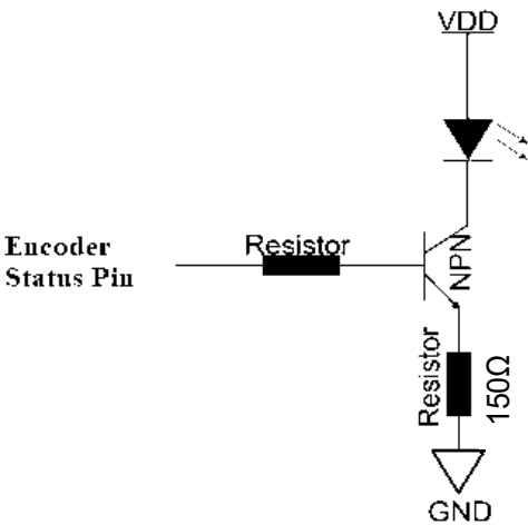
Figure 8: Status Pin Diagram
