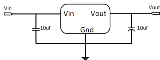
Application circuit of AF1117 fixed version
