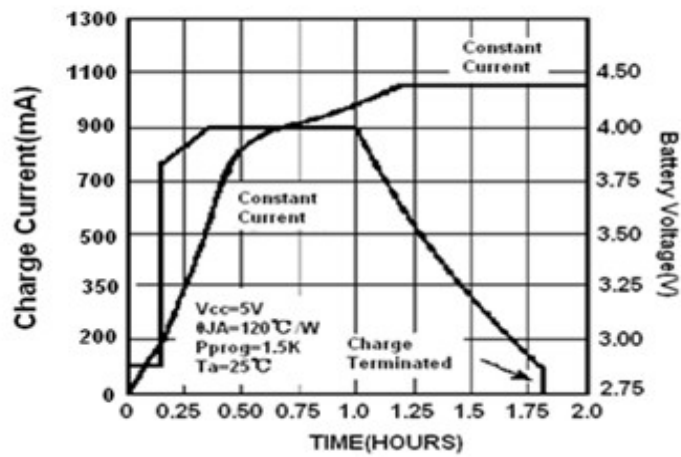
Typical charge cycle ( 1100 mAh Battery)
