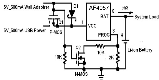
Fig.5:Combining Wall Adapter and USB Power
