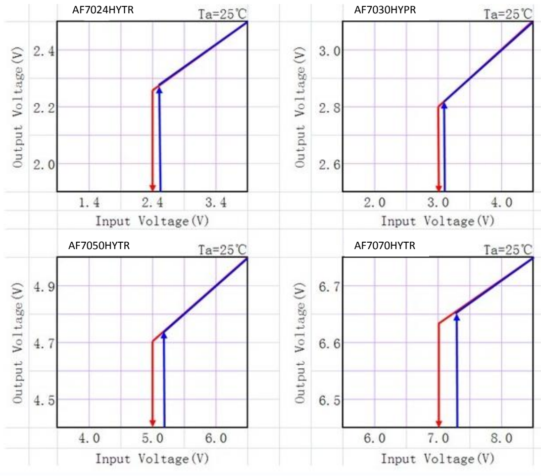
(1) Output Voltage vs Input voltage
