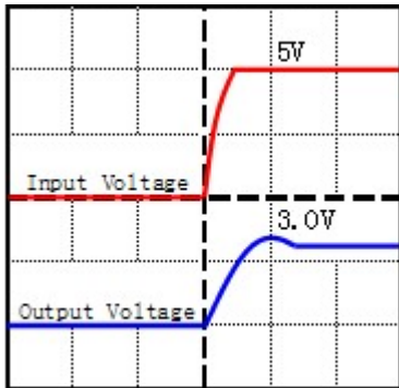
Time (5ms/div)
