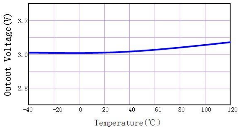
AF7330MPR Cin=CL=10uF(Electrolytic Capacitor)
