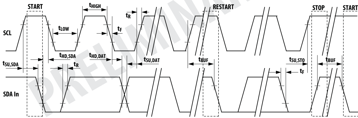
Figure 12. I2C Interface Bus Timing
