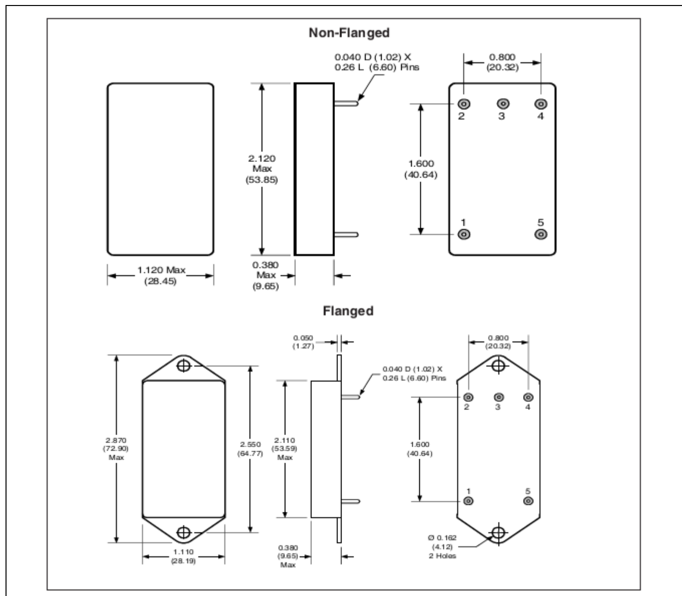
Figure 3 Package outline
