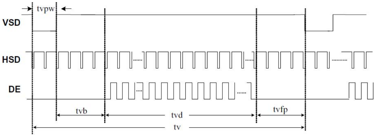
Vertical timing
