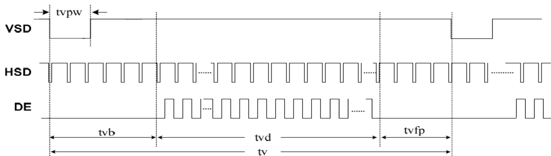
Vertical input timing
