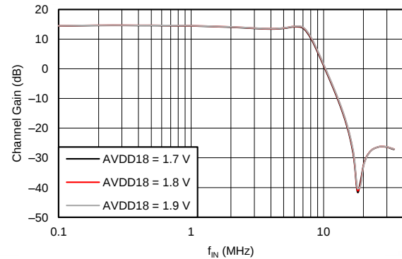
Figure 42. Antialias Filter Response vs AVDD18 (PGA Gain = 0\text{ dB} , FILTER_BW = 8\text{ MHz} )
