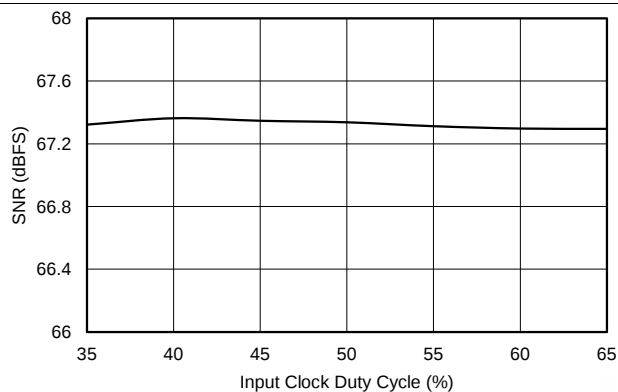
Figure 130. Signal-to-Noise Ratio vs Input Clock Duty Cycle (PGA Gain = 0 dB)
