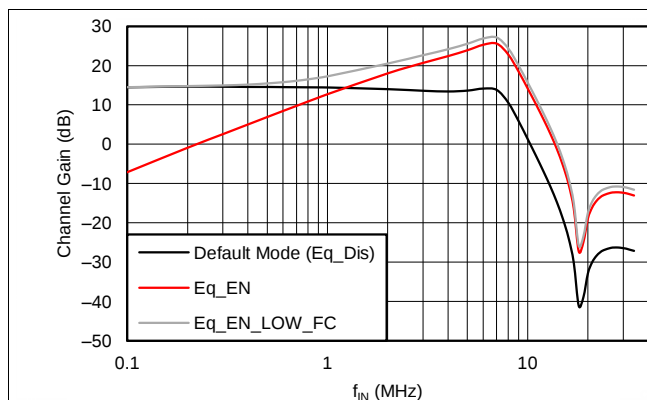
Figure 65. Filter Response (PGA Gain = 0 dB)
