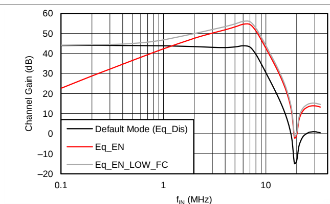
Figure 66. Filter Response (PGA Gain = 30 dB)
