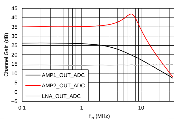
Figure 75. Frequency Response for VOUT_ON_ADC Settings (PGA Gain = 30 dB)
