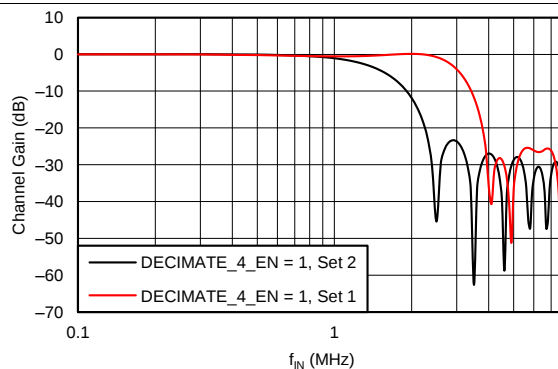
Figure 50. Decimate-by-4 Filter Response (Sampling Frequency = 12.5 MHz)
