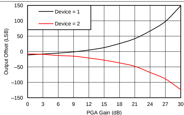
Figure 38. Channel Offset vs PGA Gain for Two Typical Devices
