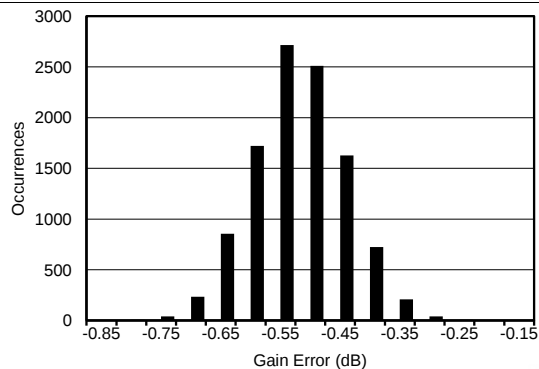
Figure 36. Gain Error Histogram for PGA Gain = 30 dB
