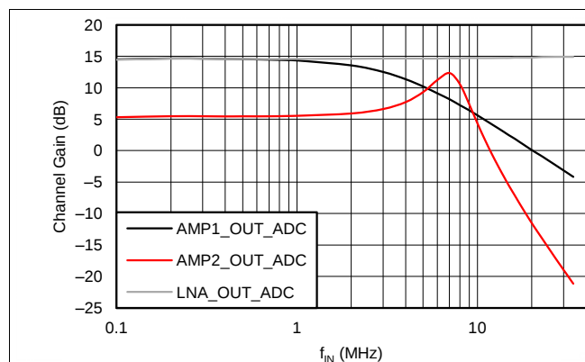
Figure 74. Frequency Response for VOUT_ON_ADC Settings (PGA Gain = 0 dB)
