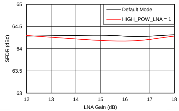
Figure 30. Spurious-Free Dynamic Range vs LNA Gain (PGA Gain = 30\text{ dB} )
