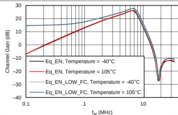
Figure 44. Antialias Filter Response for Equalizer Modes (PGA Gain = 0\text{ dB} )
