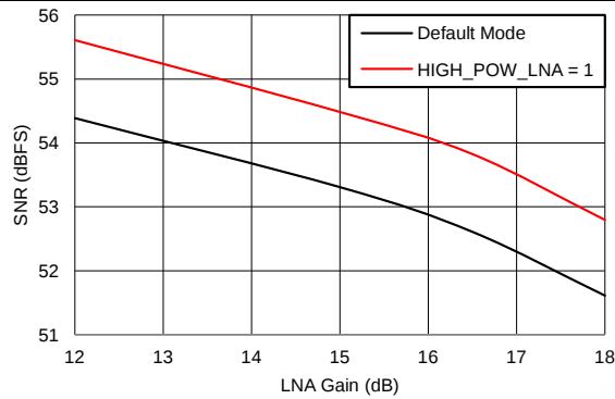
Figure 29. Signal-to-Noise Ratio vs LNA Gain (PGA Gain = 30\text{ dB} )
