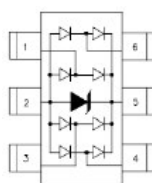
SOT-23 6L (Top View)
