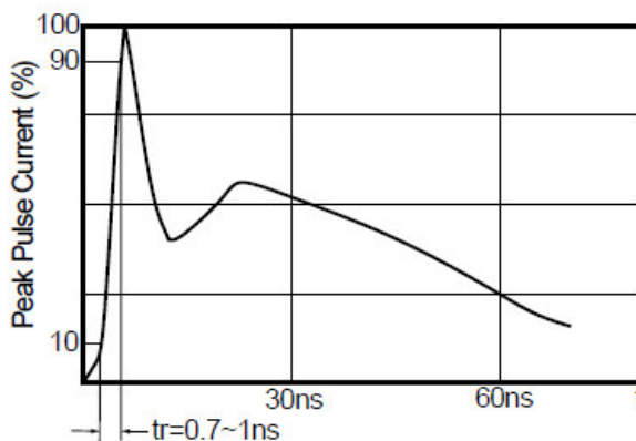
IEC61000-4-2 waveform
