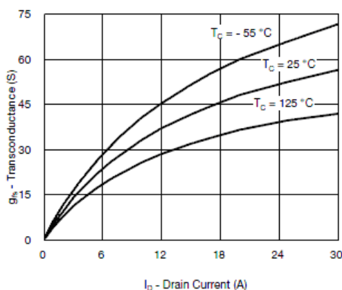
Transconductance
