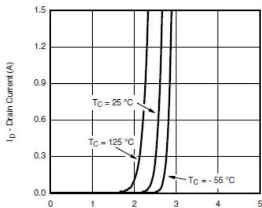
Transfer Characteristics
