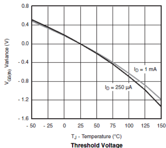
Threshold Voltage
