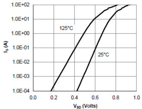
Body-Diode Characteristics
