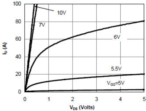
On-Region Characteristics
