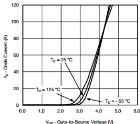
Transfer Characteristics
