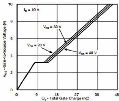
Gate Charge
