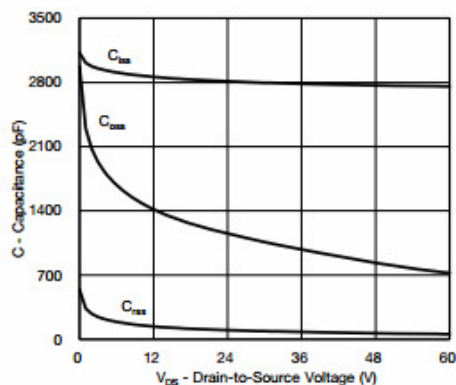
Capacitance
