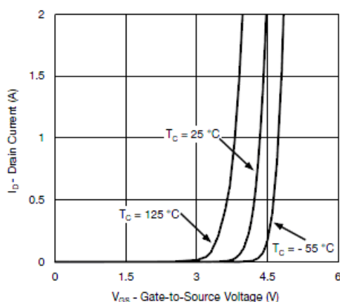
Transfer Characteristics
