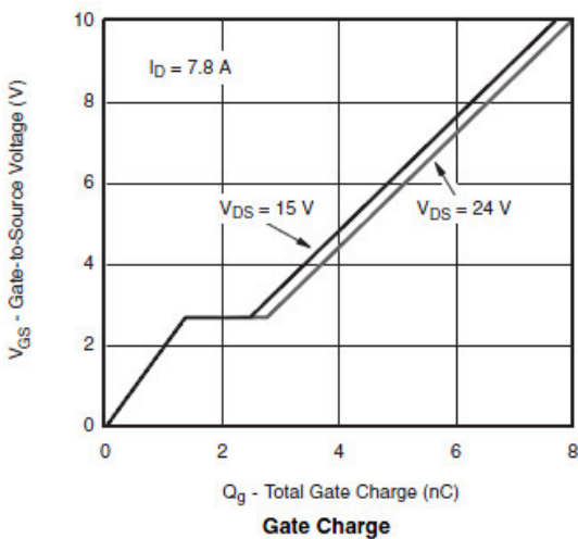
Gate Charge
