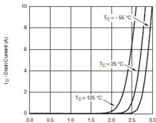
Transfer Characteristics
