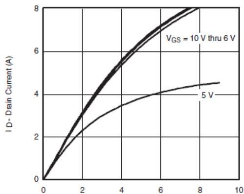
Output Characteristics
