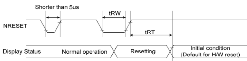
Figure 102 Reset Timing
