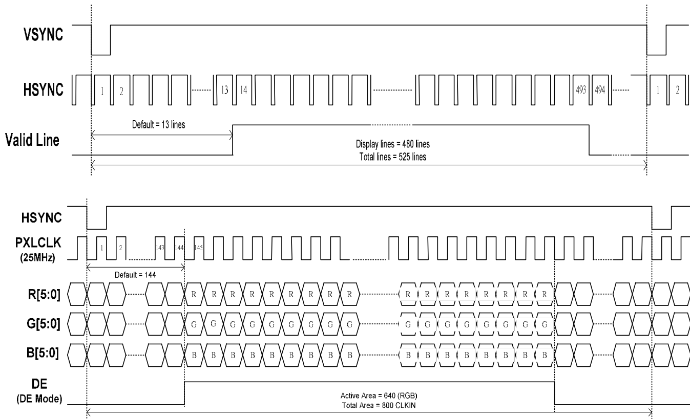
Fig. 3-4 18 bit RGB mode for 640 x (RGB) x 480
