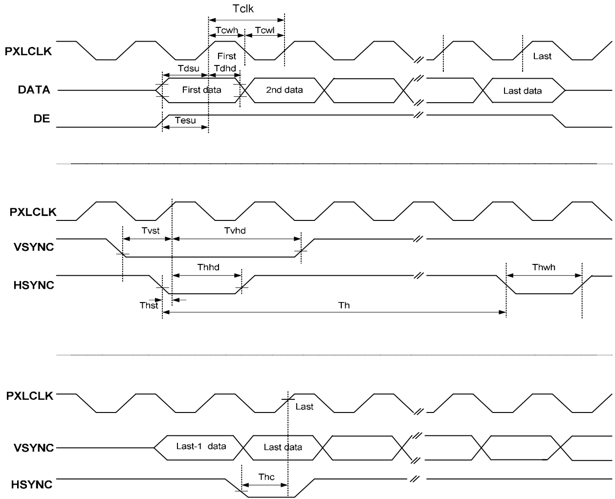
Fig.3-1 Clock and Data Input Timing Diagram
