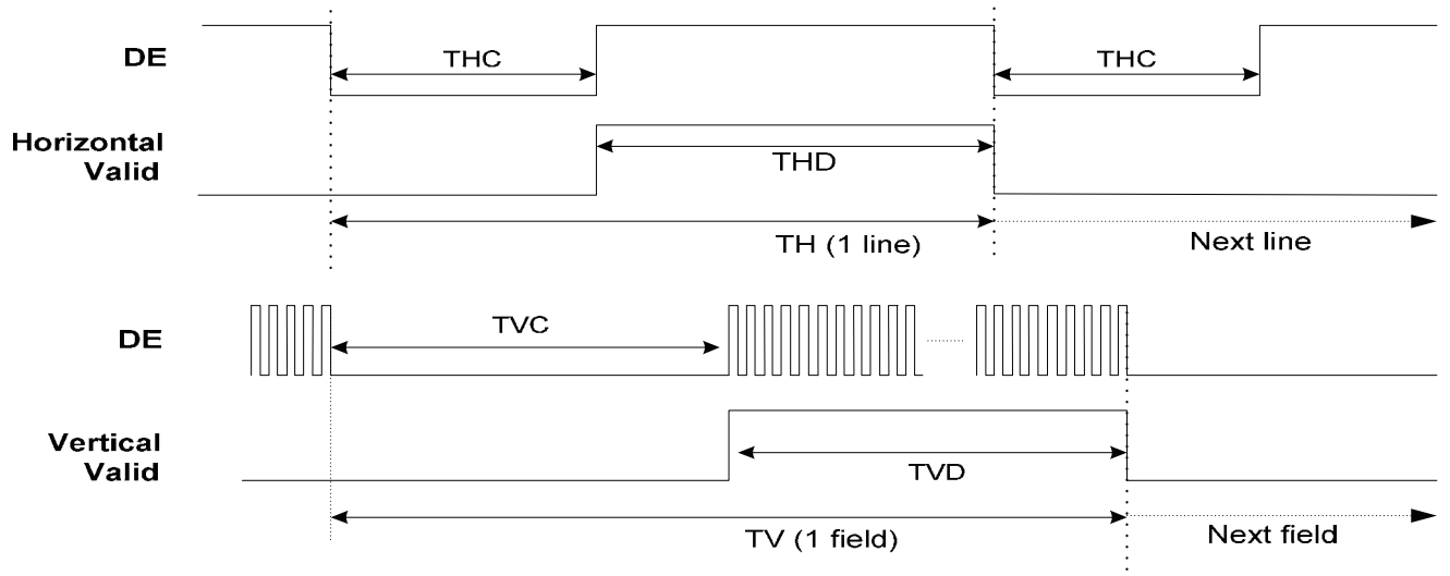
Fig.3-2 DE Mode Input Timing
