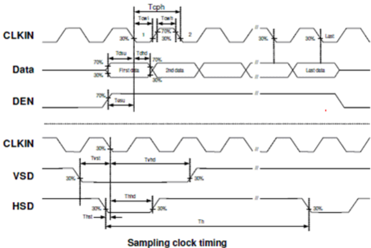
Timing Diagram of Interface Signal
