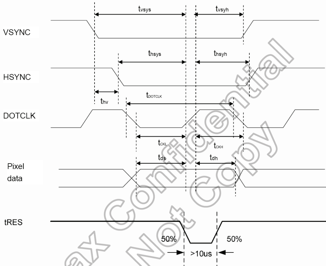
Figure 12. 1 Pixel Timing
