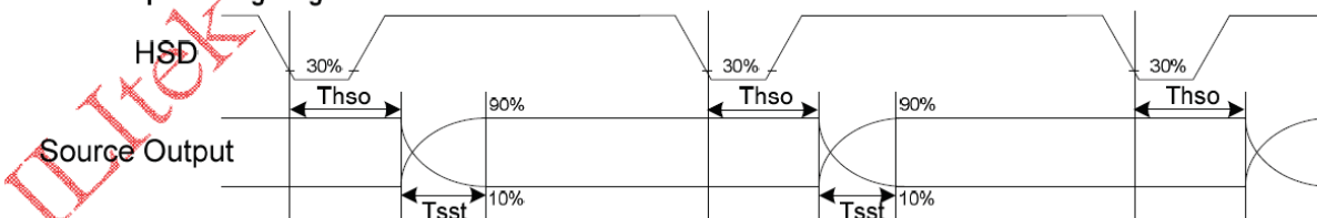
Source output timing diagram
