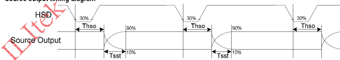
Source output timing diagram
