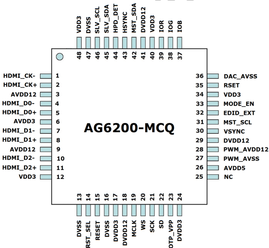
Figure 3 48-Pin Mapping
