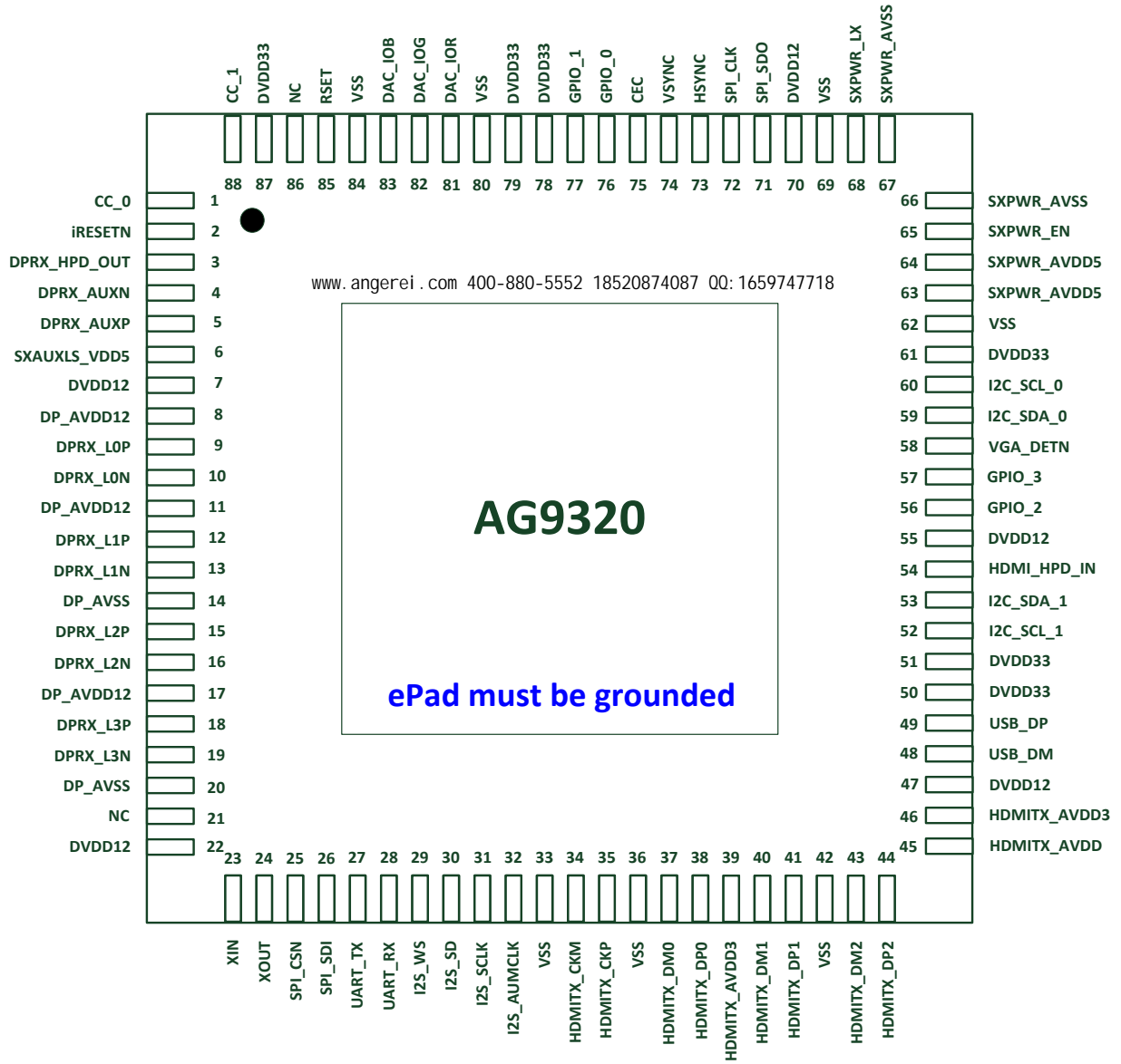
Figure 3 AG9320 PIN Mapping
