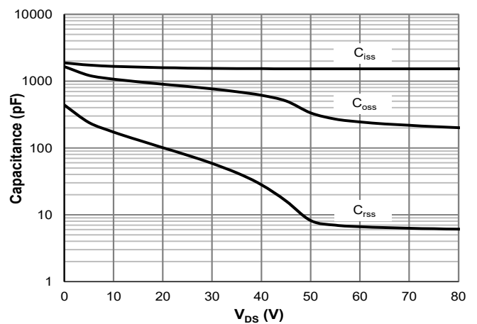
Figure 6: Capacitance Characteristics
