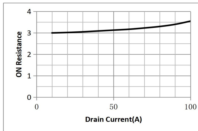
Fig.4 Resistance V.S Drain Current
