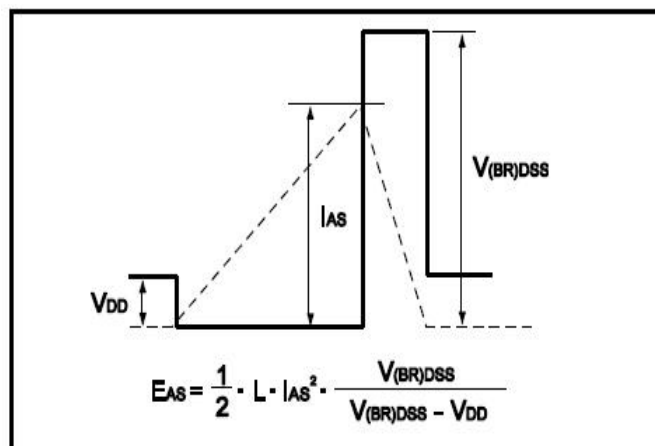
Fig.12 Avalanche Waveform
