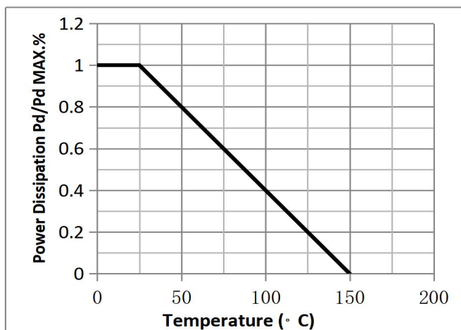
Fig.1 Power Dissipation
