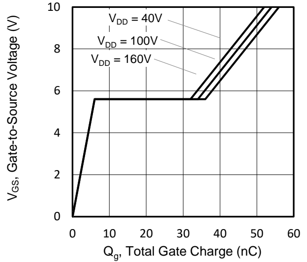
Figure 8. Gate Charge
