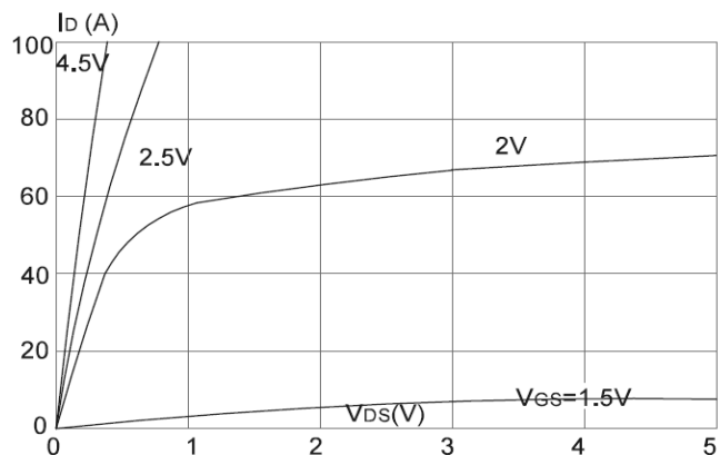
Figure1: Output Characteristics
