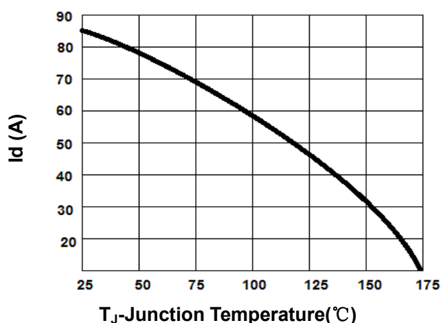
Figure 4. Drain Current
