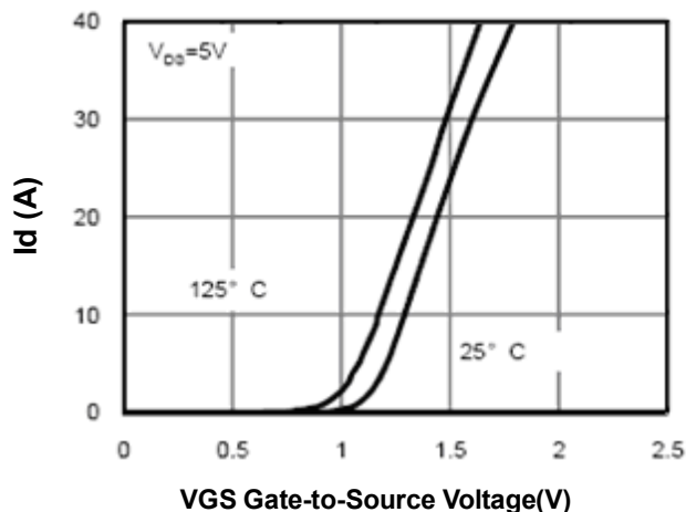
Figure 4. Drain Current
