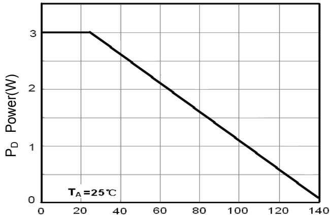
Figure 3 Power Dissipation
