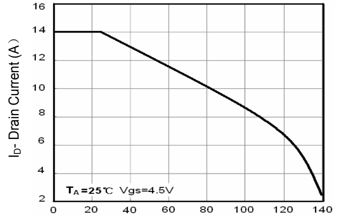
Figure 4 Drain Current
