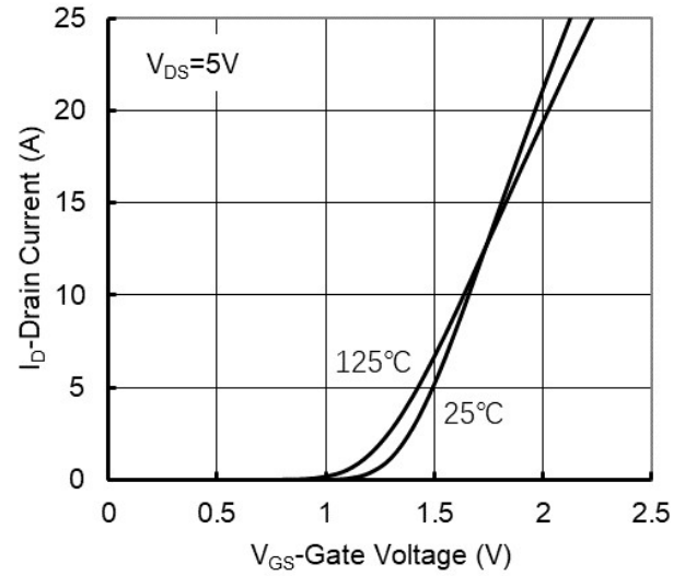
Figure2. Transfer Characteristics
