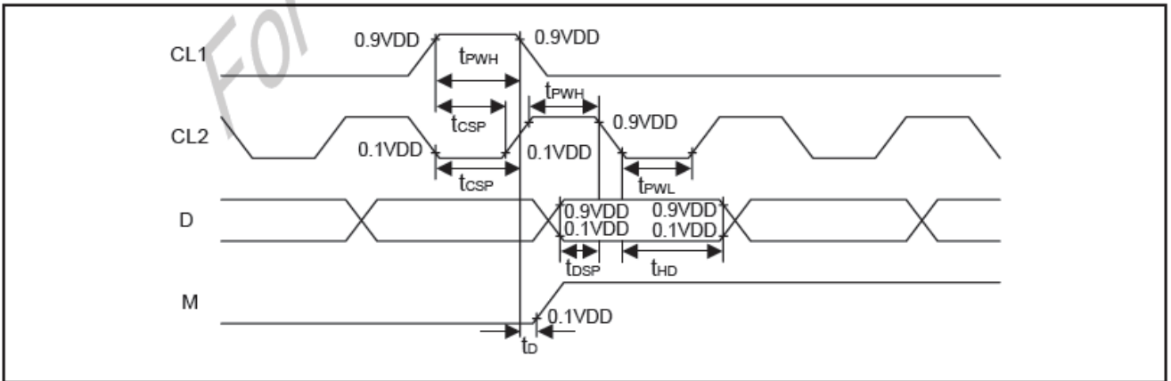
Figure 5. Interface Mode With Extension Driver Timing Diagram
