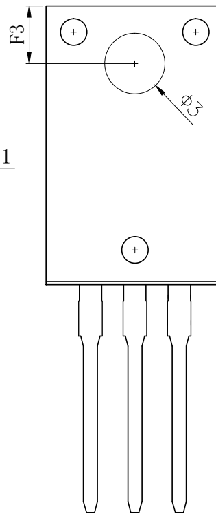
(Bottom View)
