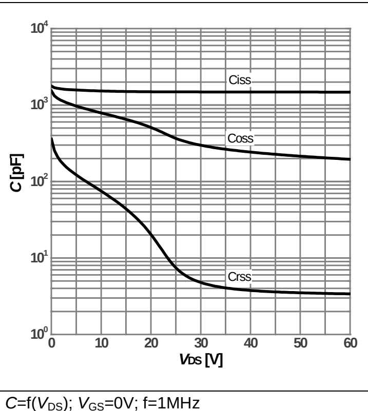
Diagram 13: Typ. capacitances
