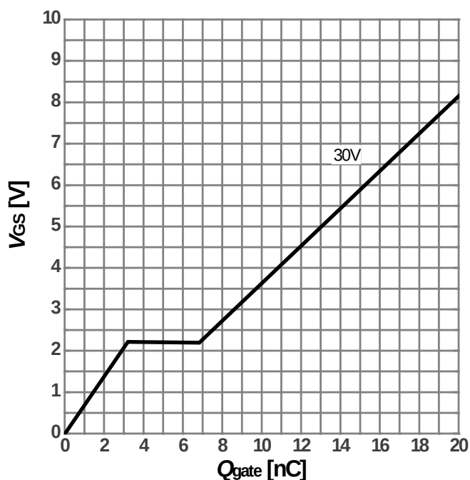
Diagram 4: Typ. gate charge
