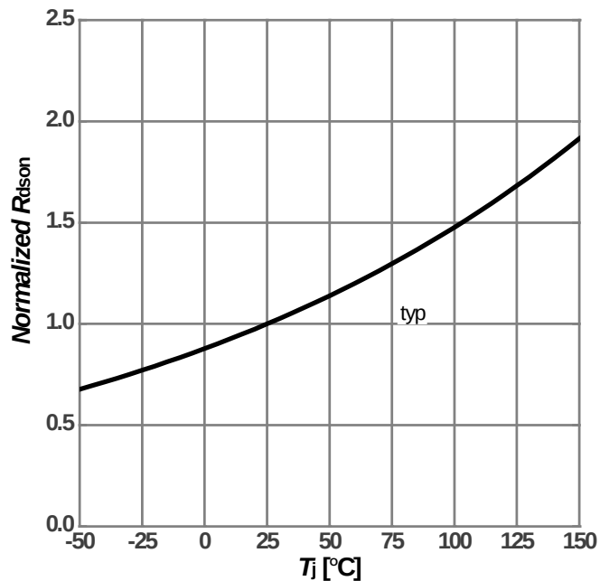
Diagram 10: On-state resistance vs. Junction temperature
