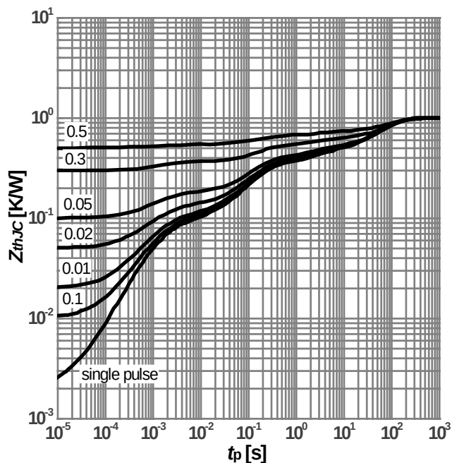
Diagram 2: Max. transient thermal impedance (SOP-8)
