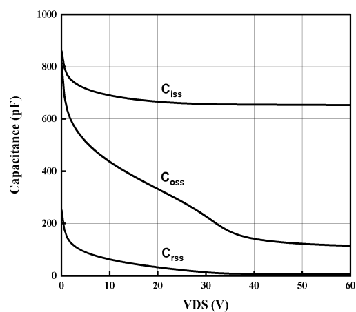
Fig5. Typical Capacitance
