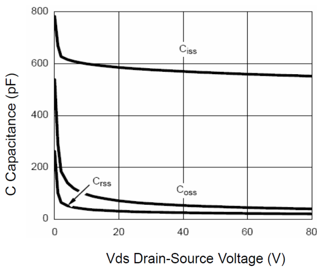
Capacitance
