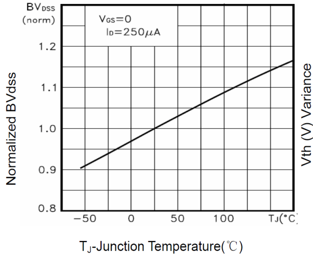
BVdss VS Junction Temperature
