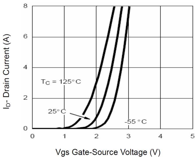
Transfer Characteristics
