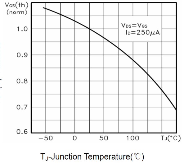
VGS vs Junction Temperature
