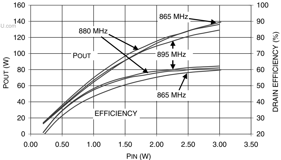
Figure 7. Power Out and Drain Efficiency vs. Input Power
