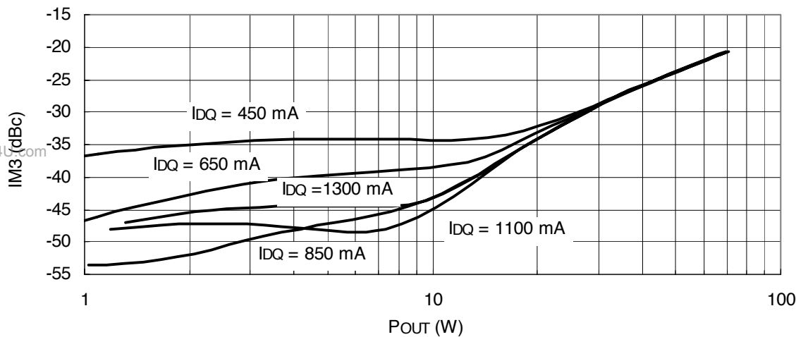
Figure 9. IM3 vs. Pout
