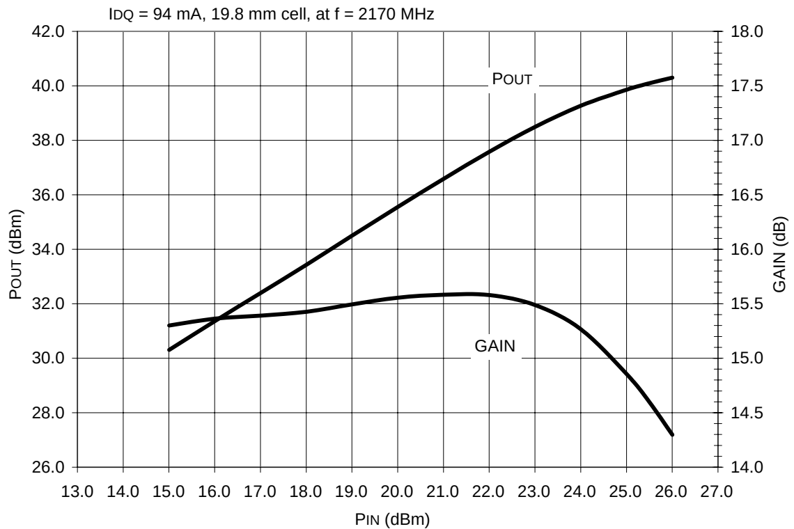
Figure 17. Gain and P_{OUT} vs. P_{IN} ( f = 2170 \text{ MHz} )
