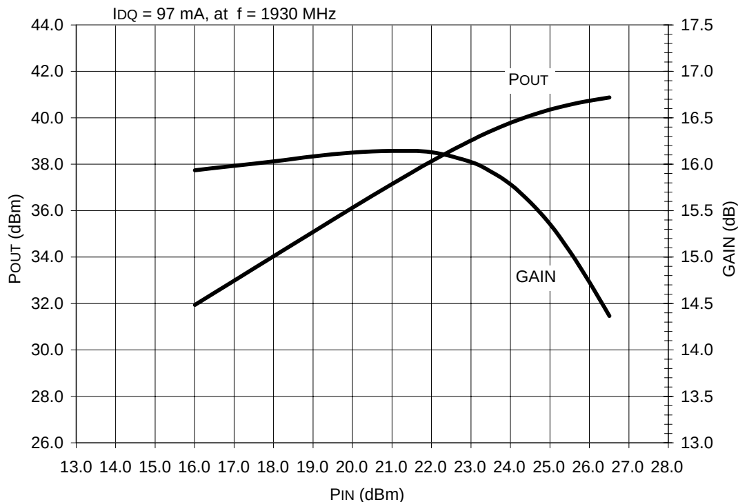
Figure 10. Gain and P_{OUT} vs. P_{IN} ( f = 1930 \text{ MHz} )
