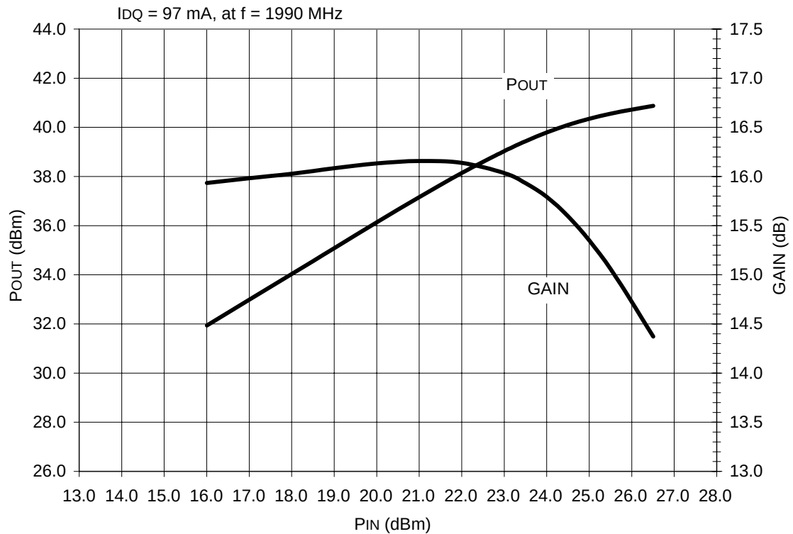
Figure 12. Gain and POUT vs. PIN ( f = 1990 \text{ MHz} )
