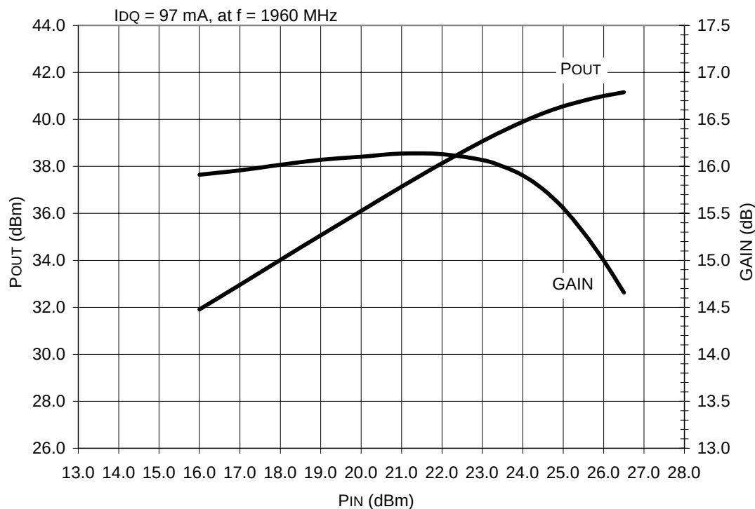
Figure 11. Gain and P_{OUT} vs. P_{IN} ( f = 1960 \text{ MHz} )
