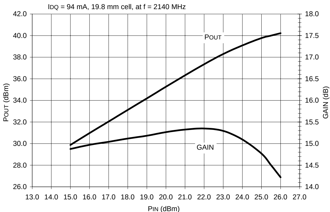
Figure 16. Gain and P_{OUT} vs. P_{IN} ( f = 2140 \text{ MHz} )
