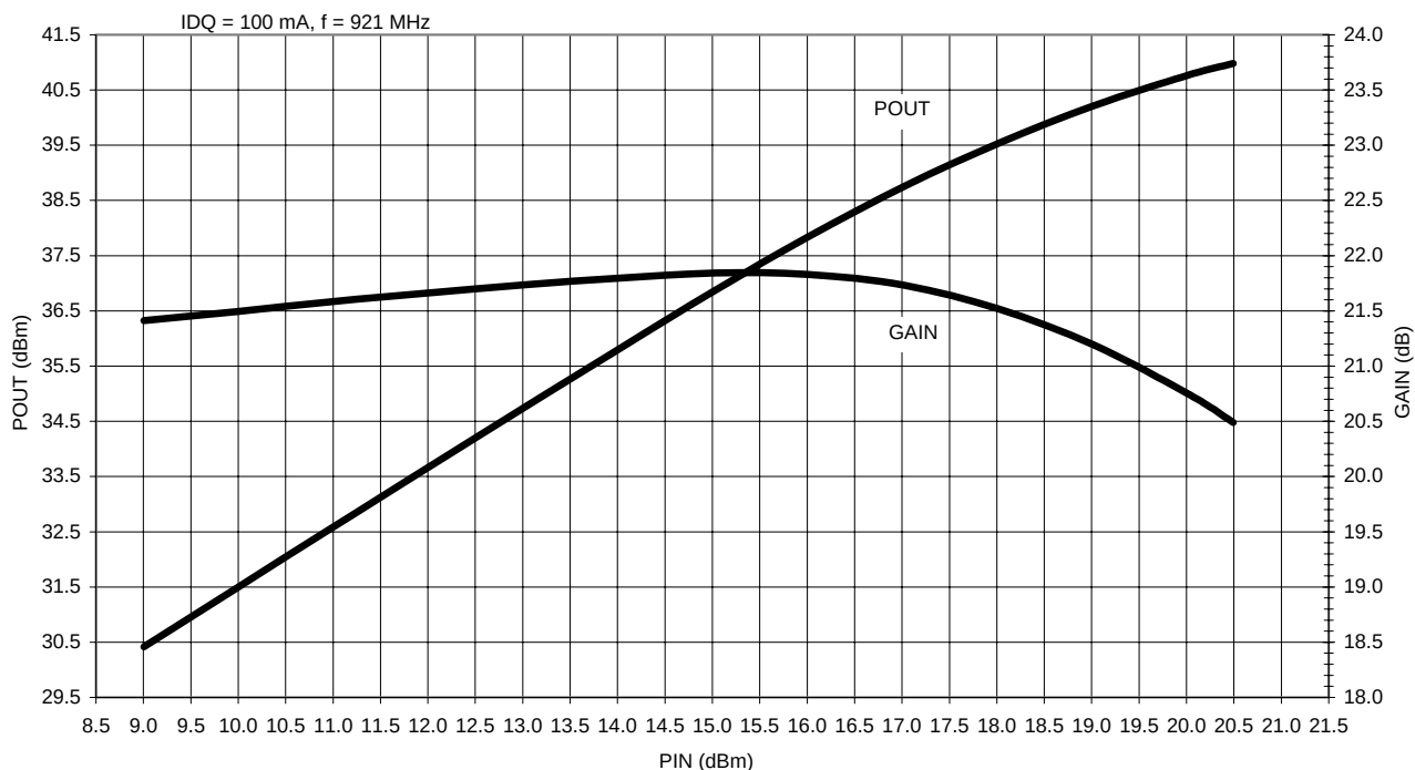
Figure 4. Gain and POUT vs. PIN (f = 921 MHz)
