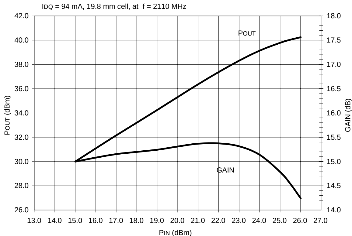
Figure 15. Gain and P_{OUT} vs. P_{IN} ( f = 2110 \text{ MHz} )
